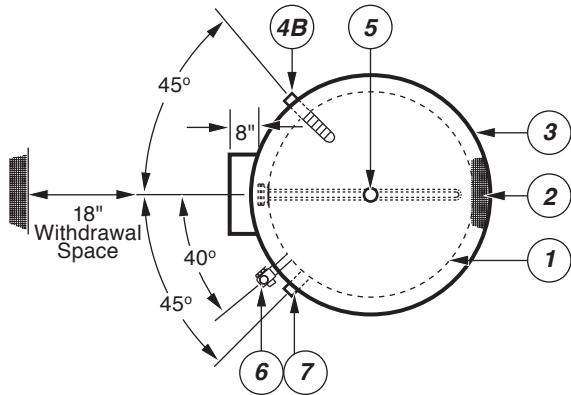
Top View - 1 1/2" Inlet/Outlet Models
